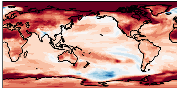
IPSL-CM5A-MR
